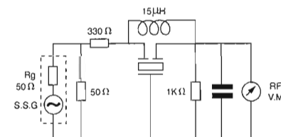
XT4.5MB测试电路TEST CIRCUIT
