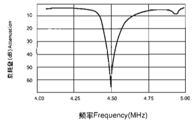
XT4.5MB频率特性Frequency Characteristics
